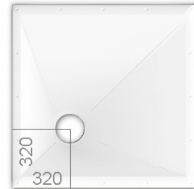
Wetroom Floor Former 900 x 900mm - 22mm Depth
